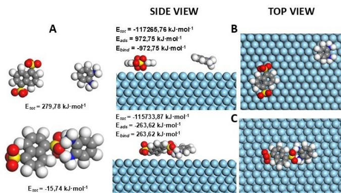
Figure 7 – View of binary system of pair of 1,2-PDAH 2 2+ and 1,5-NDS 2- at 1 : 1 ratio as individual components and hydrogen-bonded ion pair (A), and side and top views of the most appropriate configuration for adsorption of system of individual inhibitor components (B) and hydrogen-bonded ion pair (C) on Fe(110) surface.
